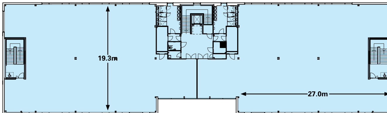
typical floor plan upper floor
